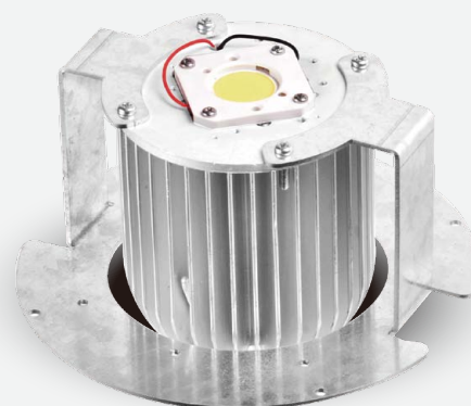
51-D009+Q 40W LED MODEL
